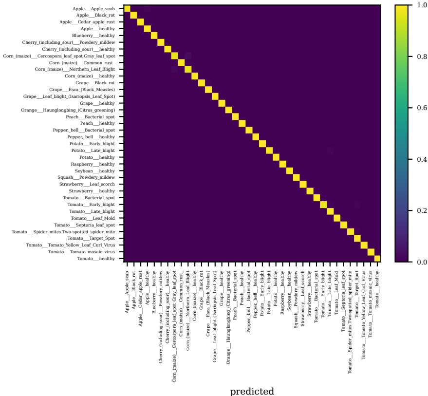
pv_resnet50_s2026 — in_domain_test (row-normalised)
