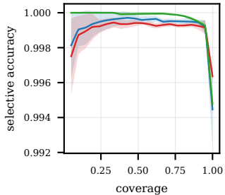
PlantVillage in-domain
