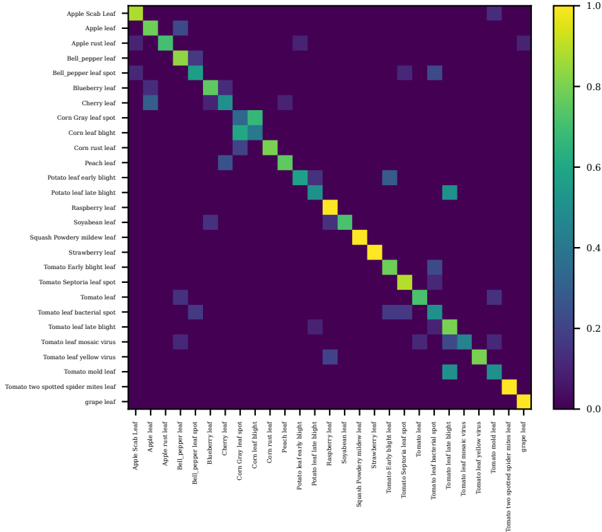
pdc_efficientnet_b0_s42 — in_domain_test (row-normalised)
