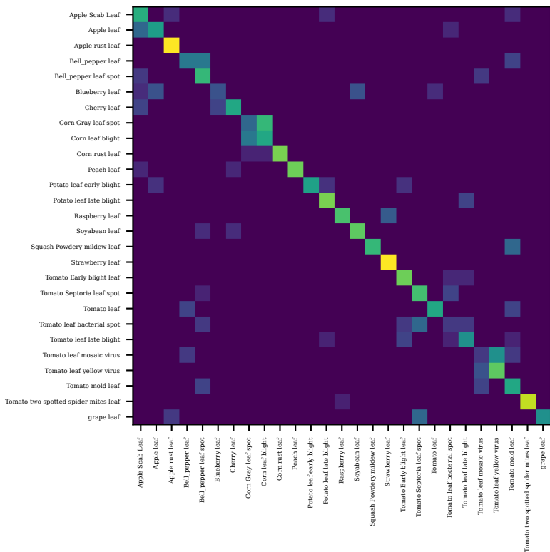
pdc_mobilenet_v3_small_s2026 — in_domain_test (row-normalised)
