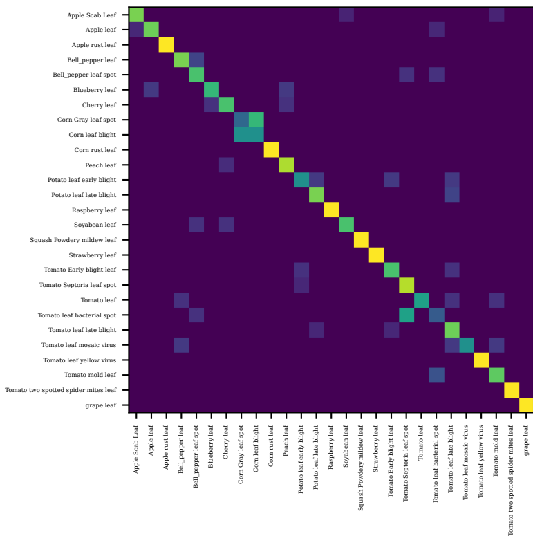
pdn_resnet50_s1337 — in_domain_test (row-normalised)
