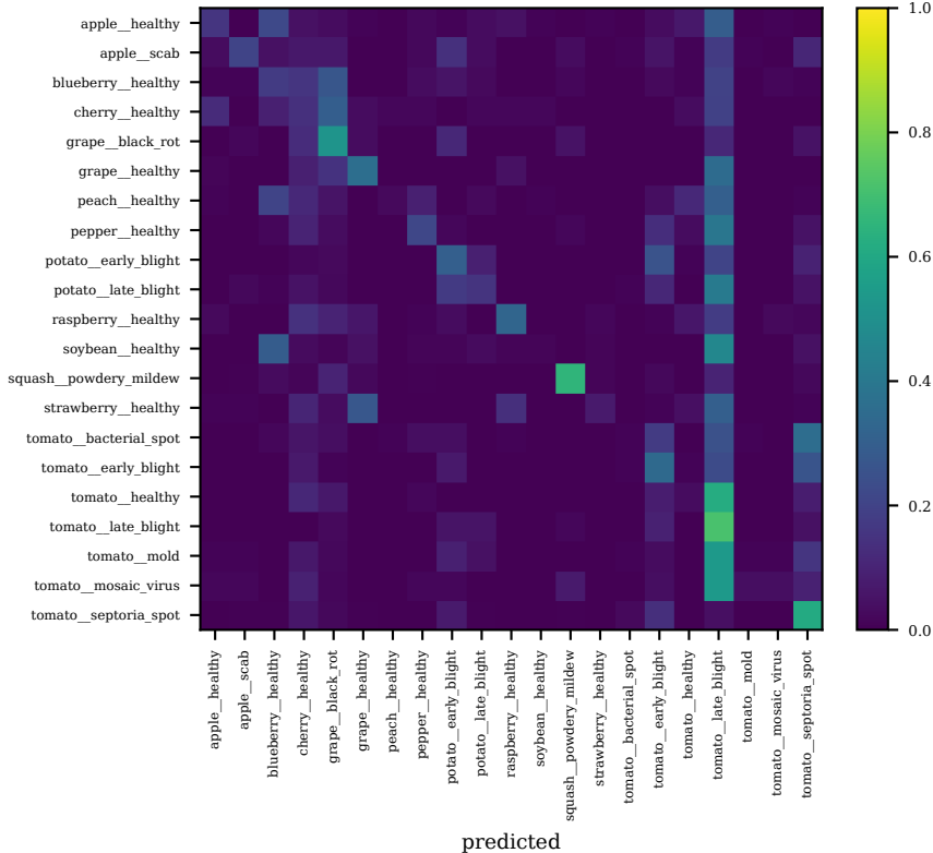
pv_efficientnet_b0_s2026 — cross_domain_plantdoc_core (row-normalised)
