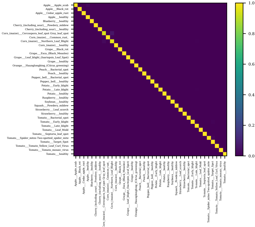
pv_efficientnet_b0_s42 — in_domain_test (row-normalised)
