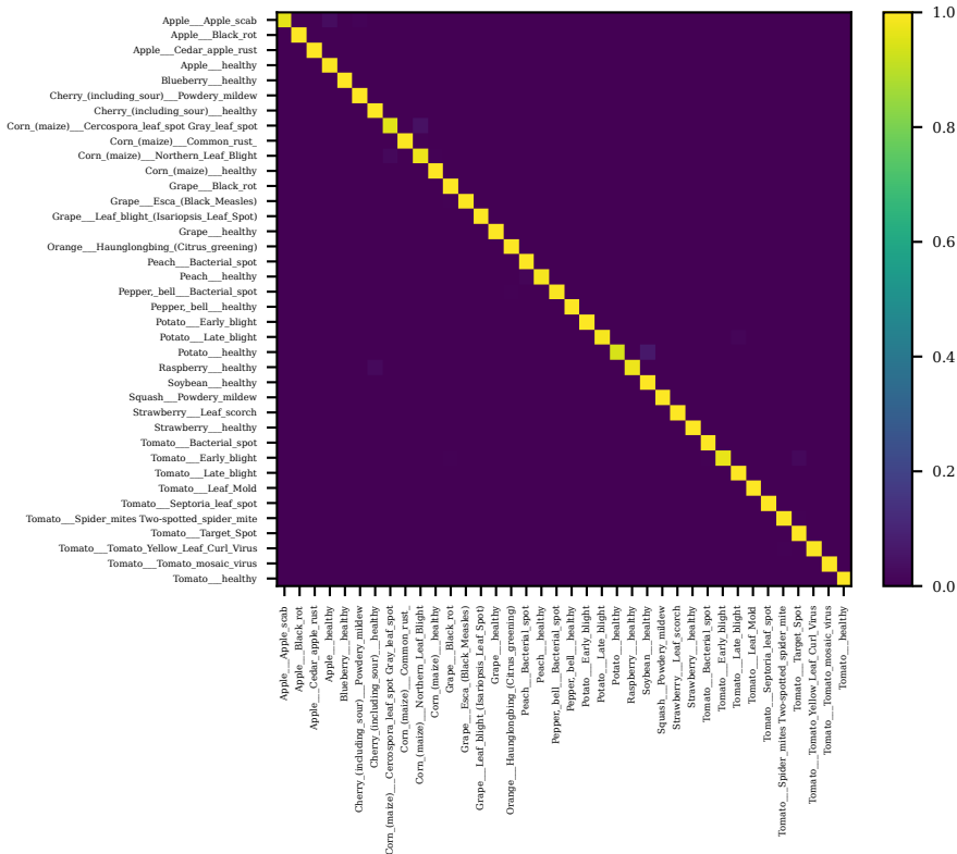
pv mobilenet v3 small s42 — in domain test (row-normalised)
