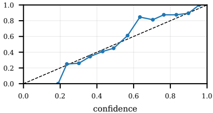
in_domain_test_temperature_scaled ECE=0.0545
