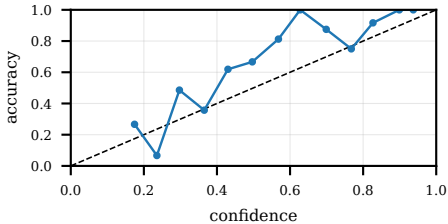
in_domain_test ECE=0.1536
