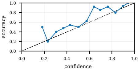
in_domain_test ECE=0.1071
