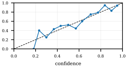
in_domain_test_temperature_scaled ECE=0.0618
