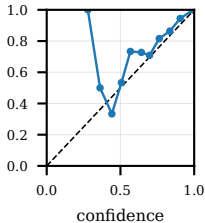
in_domain_test_temperature_scaled ECE=0.0090
