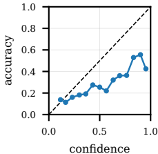
cross_domain_plantdoc_core ECE=0.1594
