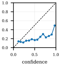
cross_domain_plantdoc_core ECE=0.3013
