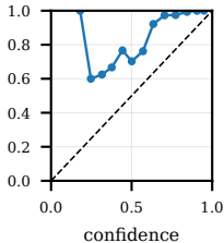
in_domain_test ECE=0.0989
