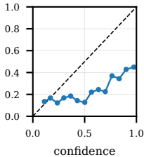
cross_domain_plantdoc_core ECE=0.3011
