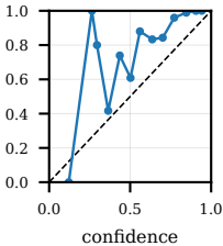
in_domain_test ECE=0.0962
