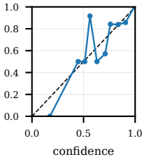
in_domain_test_temperature_scaled ECE=0.0089
