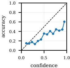
cross_domain_plantdoc_core ECE=0.1600
