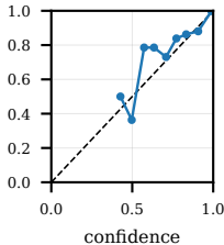
in_domain_test_temperature_scaled ECE=0.0101
