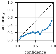
cross_domain_plantdoc_core ECE=0.3146
