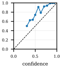
in_domain_test ECE=0.1116
