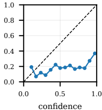
cross_domain_plantdoc_core_temperature_scaled ECE=0.4636
