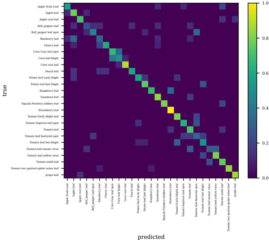
pdn_mobilenet_v3_small_s42 — in_domain_test (row-normalised)
