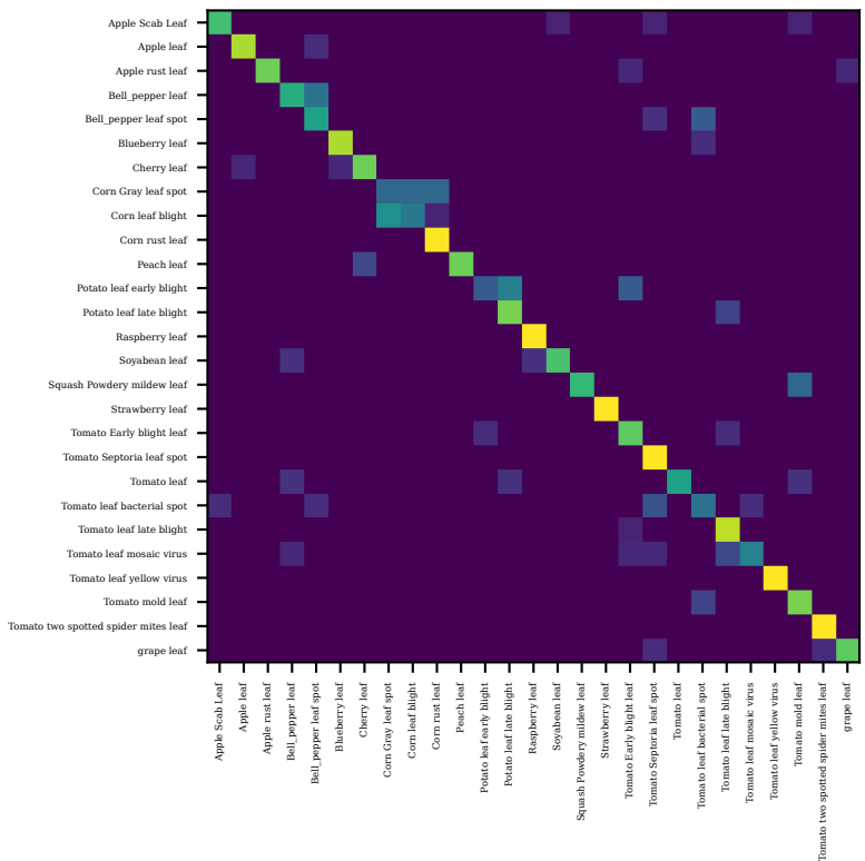
pdc_resnet50_s42 — in_domain_test (row-normalised)
