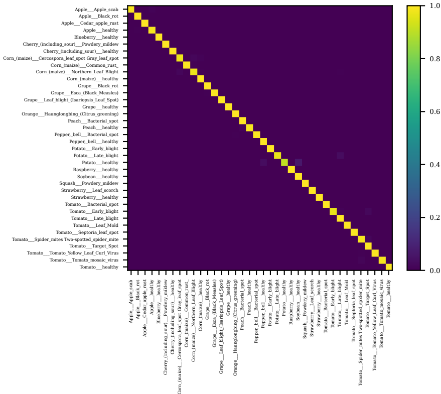
pv_mobilenet_v3_small_s1337 — in_domain_test (row-normalised)
