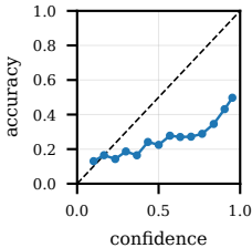
cross_domain_plantdoc_core ECE=0.3038
