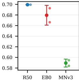
PlantDoc Core in-domain
