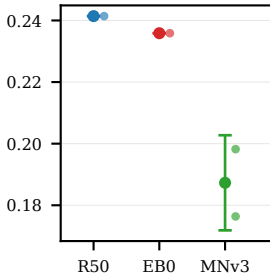
PlantVillage \rightarrow PlantDoc Core
