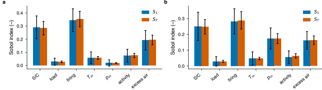
Figure 6: First-order ( S_1 ) and total-effect ( S_T ) Sobol indices with 95 % confidence intervals for (a) the hot-spot temperature and (b) \log_{10} t_r at the hot spot, from the Saltelli design of Table S8.
