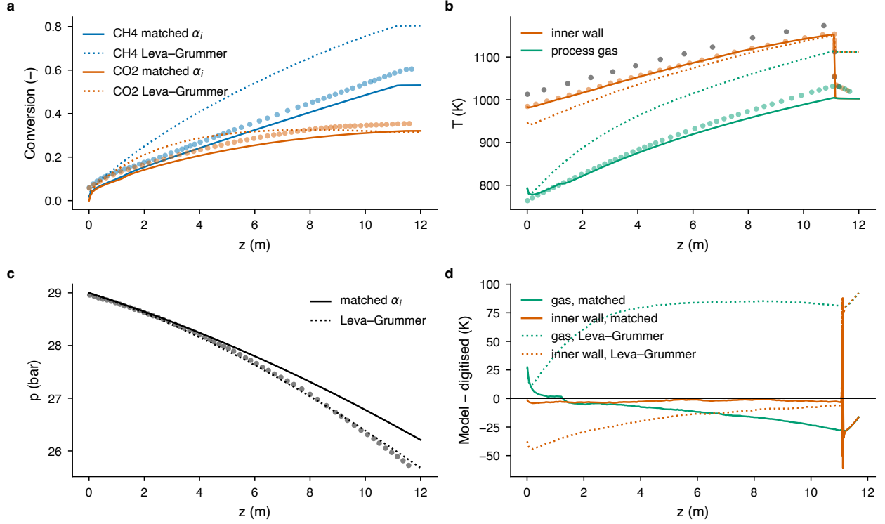
Figure 2: Verification against the digitized industrial case of Xu and Froment [6] (symbols) with the digitized outer-wall temperature as boundary condition: (a) methane and \text{CO}_2 conversion, (b) process-gas and inner-wall temperatures, (c) pressure and (d) temperature residuals, for the matched film coefficient (solid lines) and for the Leva-Grummer correlation with f_{\text{htg}} = 1 (dotted).
