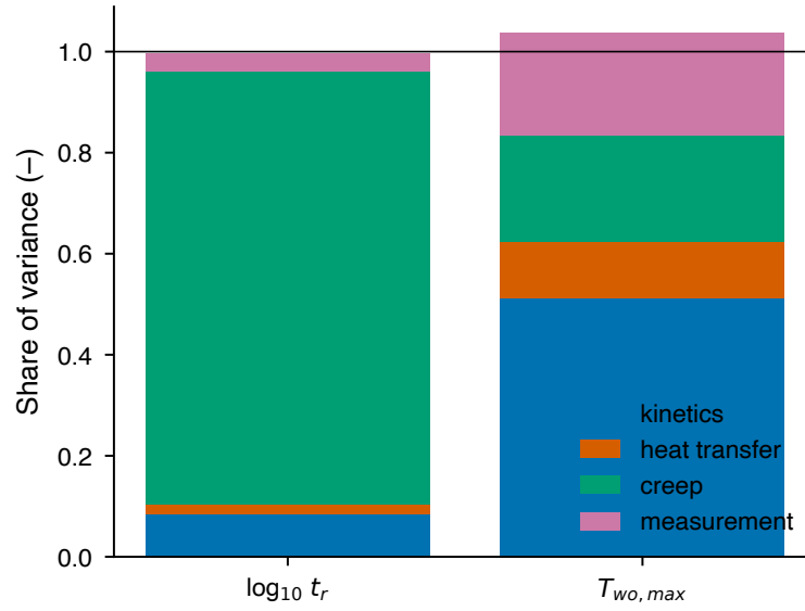
Figure S2: One-group-at-a-time shares of the variance of \log_{10} t_r and of the hot-spot temperature at the S1 base point; numerical values in Table S7.
