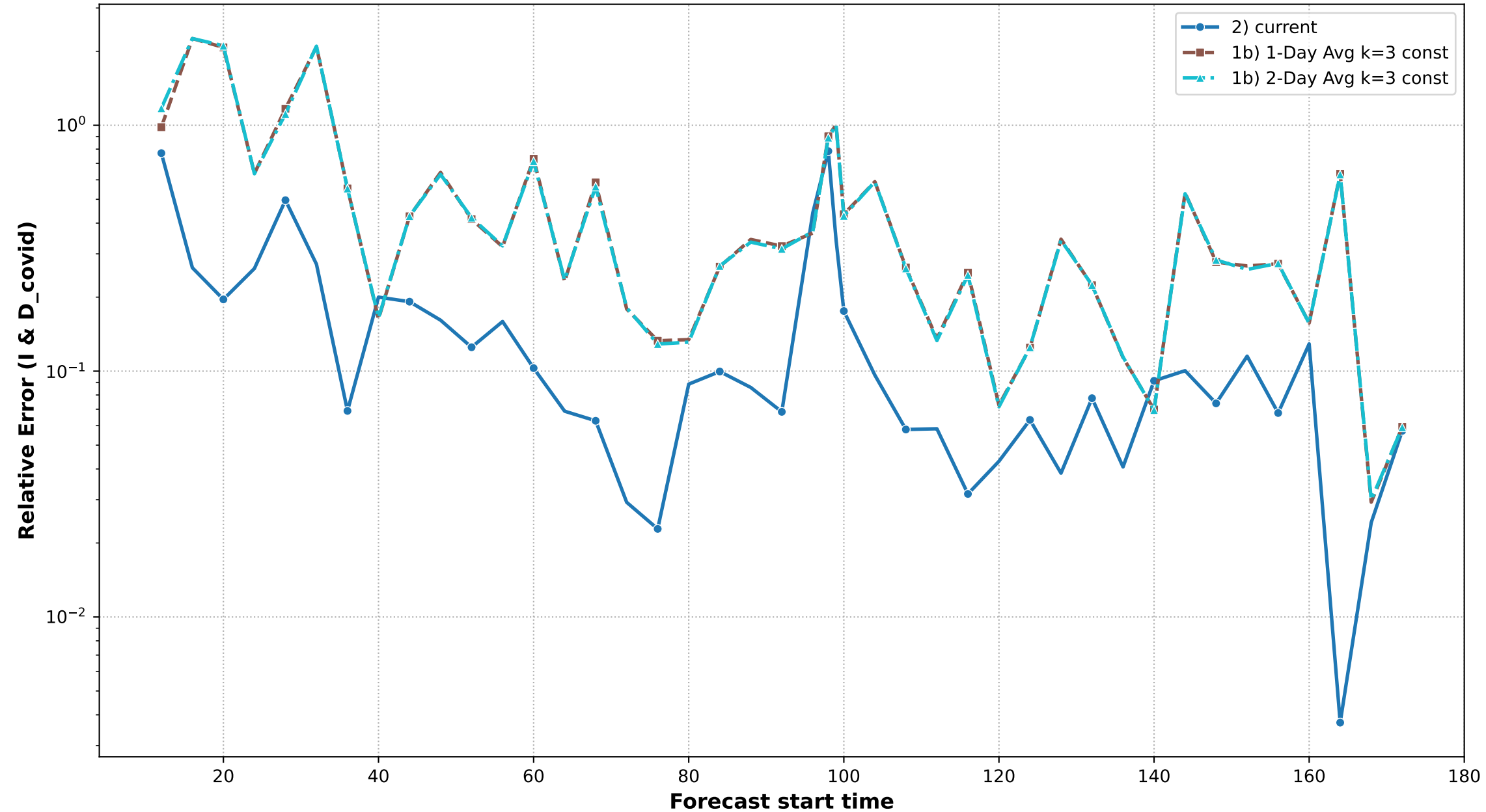
Rolling Forecast Performance (7.0 Days, I and D_covid vs Numerical Reference)
