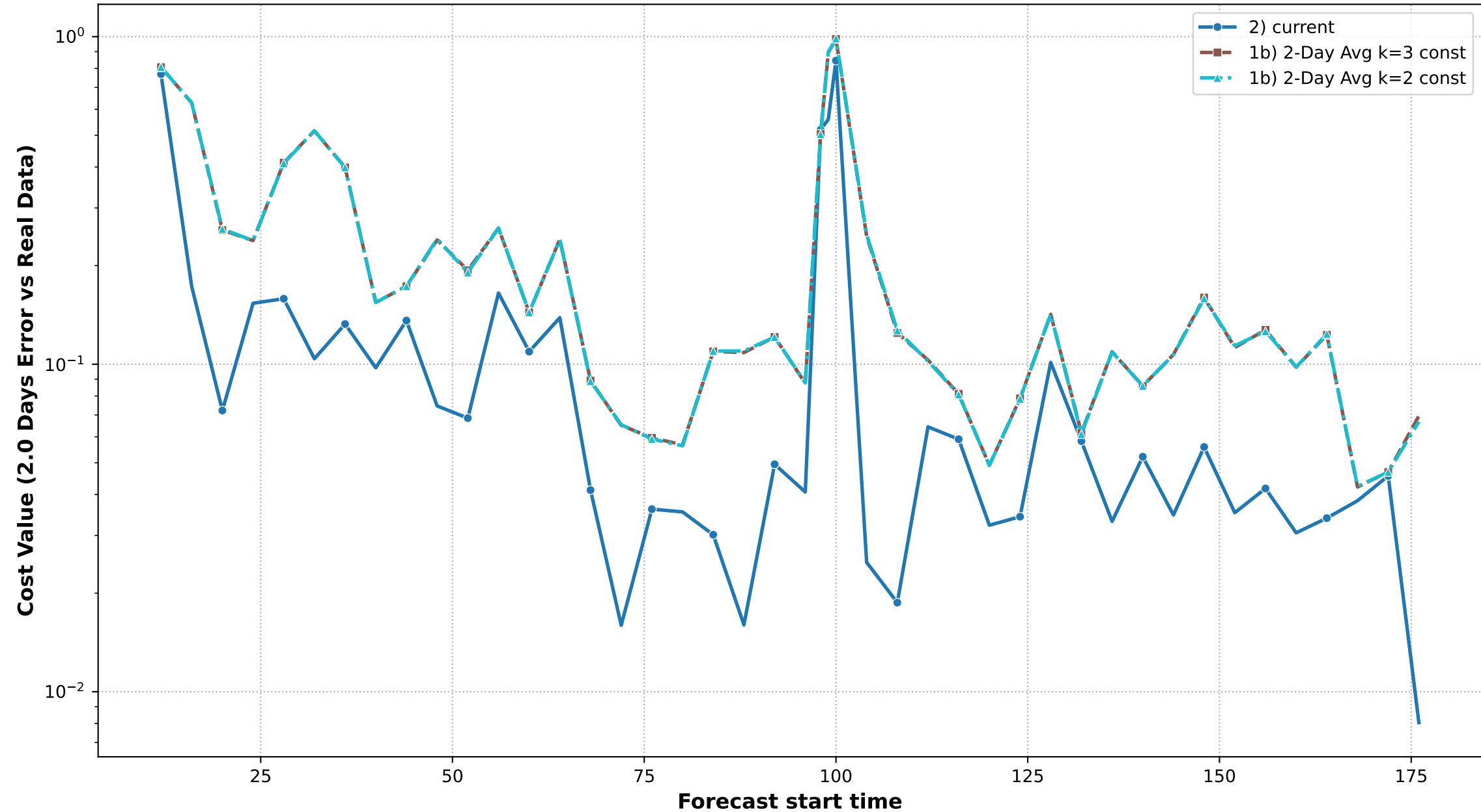
Rolling Forecast Performance (2.0 Days vs Real Data)
