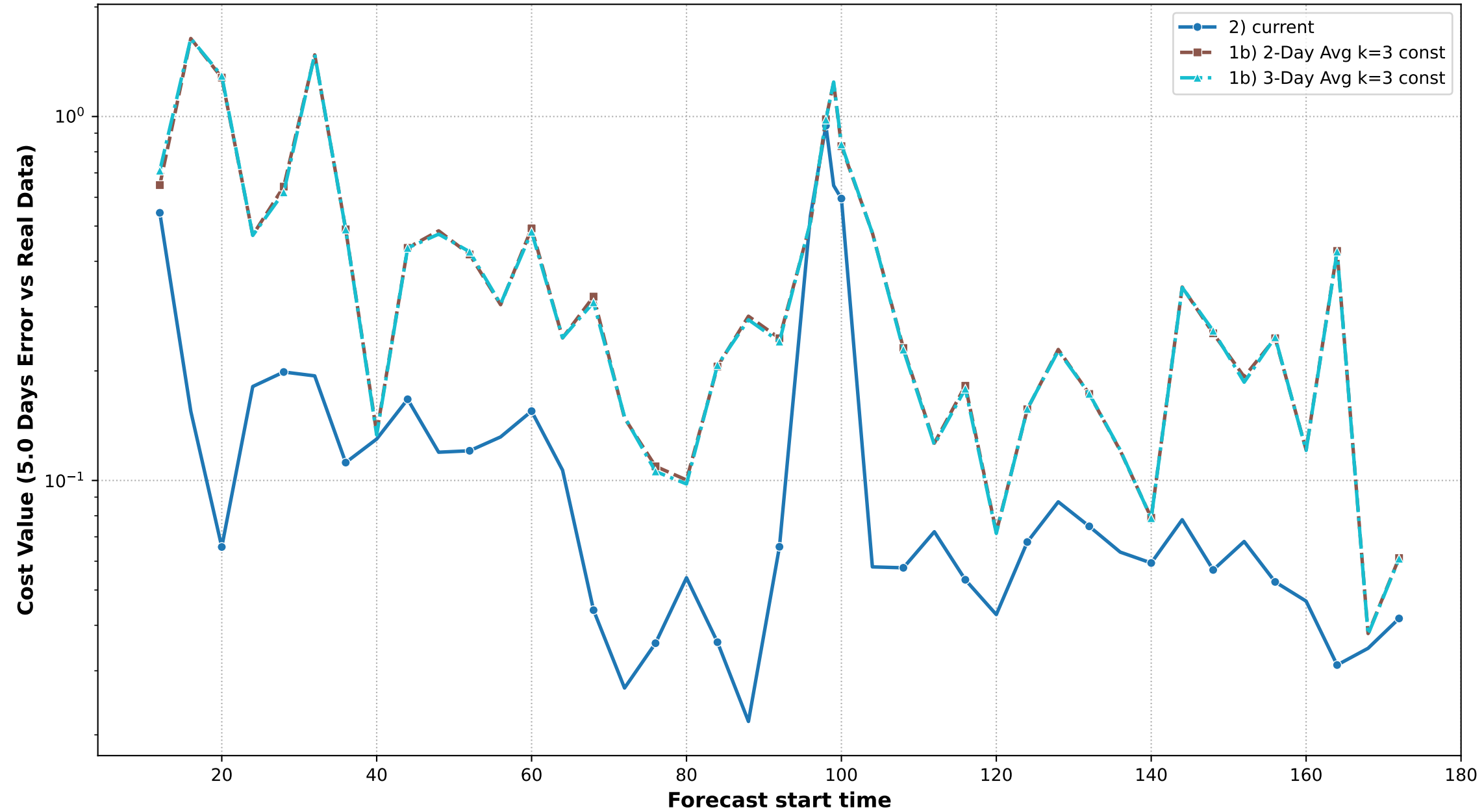
Rolling Forecast Performance (5.0 Days vs Real Data)
