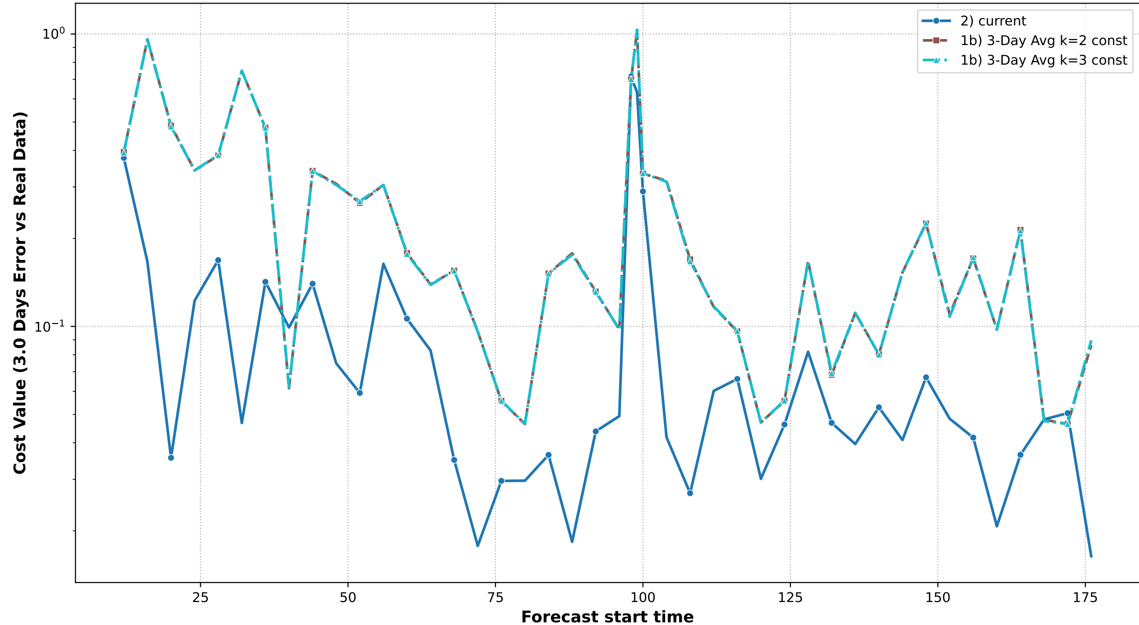
Rolling Forecast Performance (3.0 Days, u_0 shifted to match real data, S compensates)
