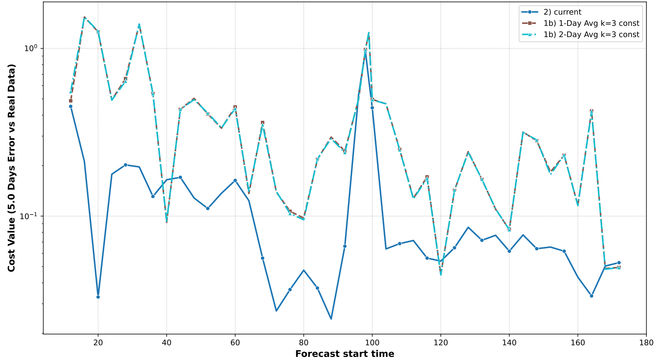
Rolling Forecast Performance (5.0 Days, u_0 shifted to match real data, S compensates)
