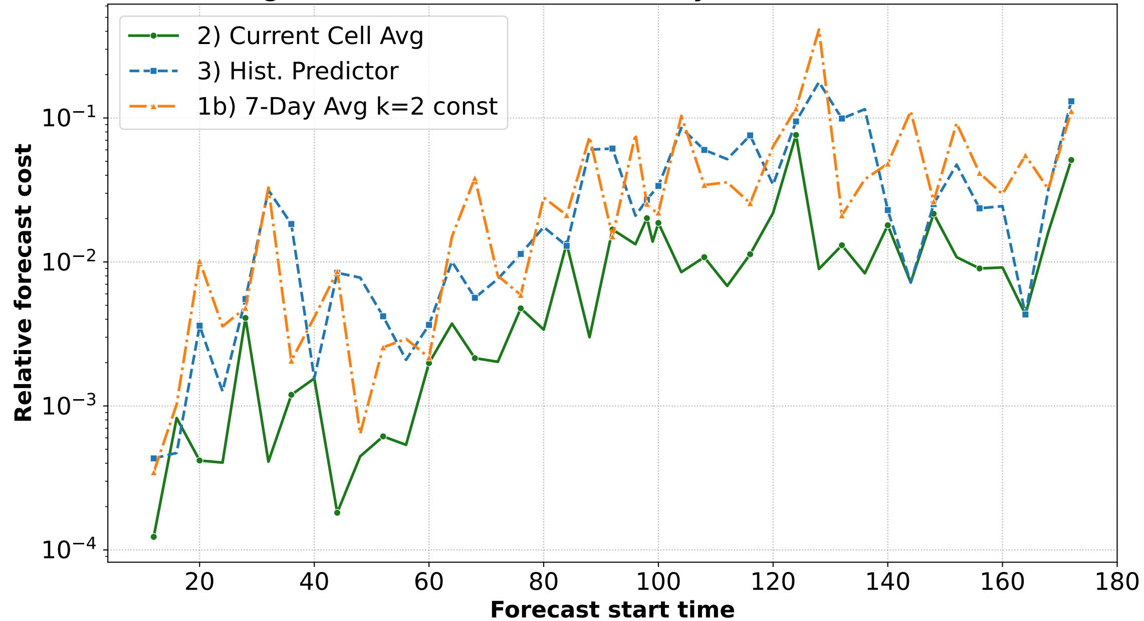
Rolling Forecast Performance (7.0 Days vs Reference Solution)
