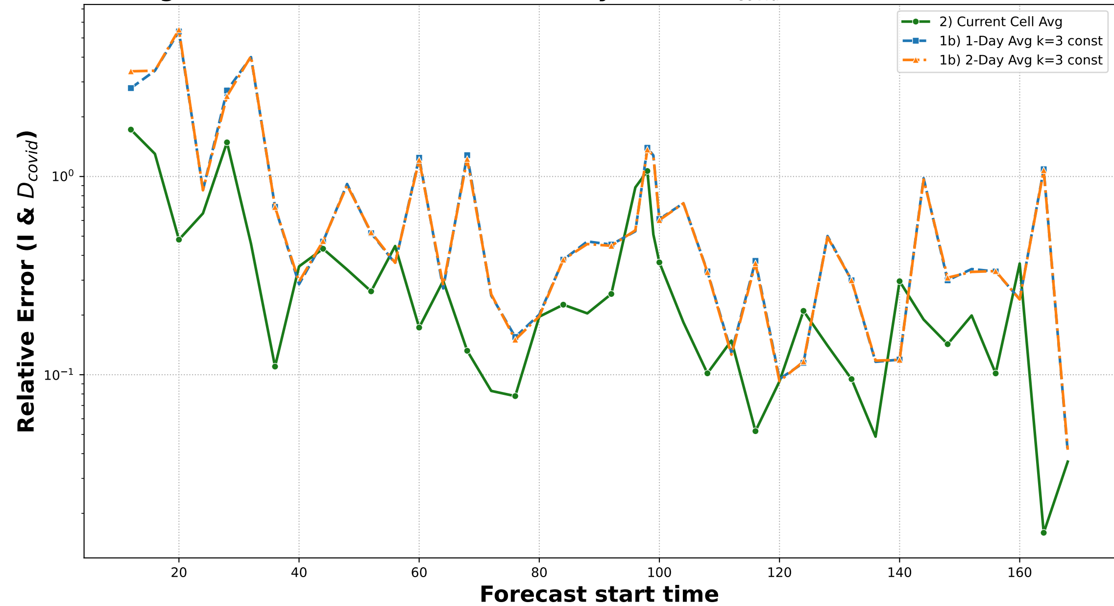
Rolling Forecast Performance (10.0 Days, I and D_{covid} vs Numerical Reference)
