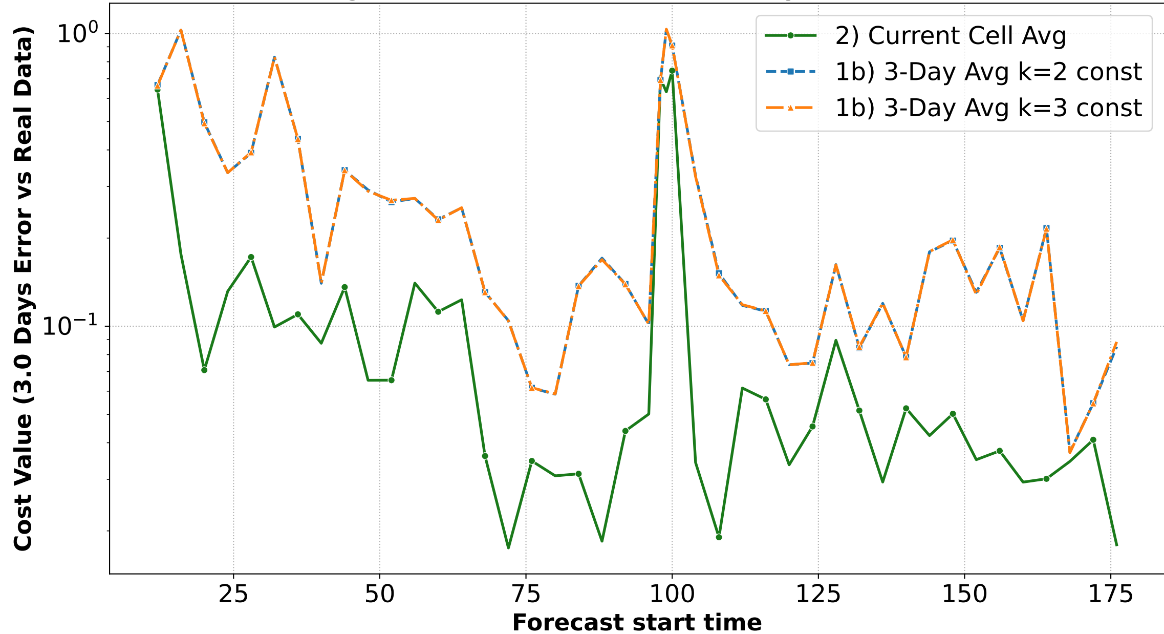
Rolling Forecast Performance (3.0 Days vs Real Data)
