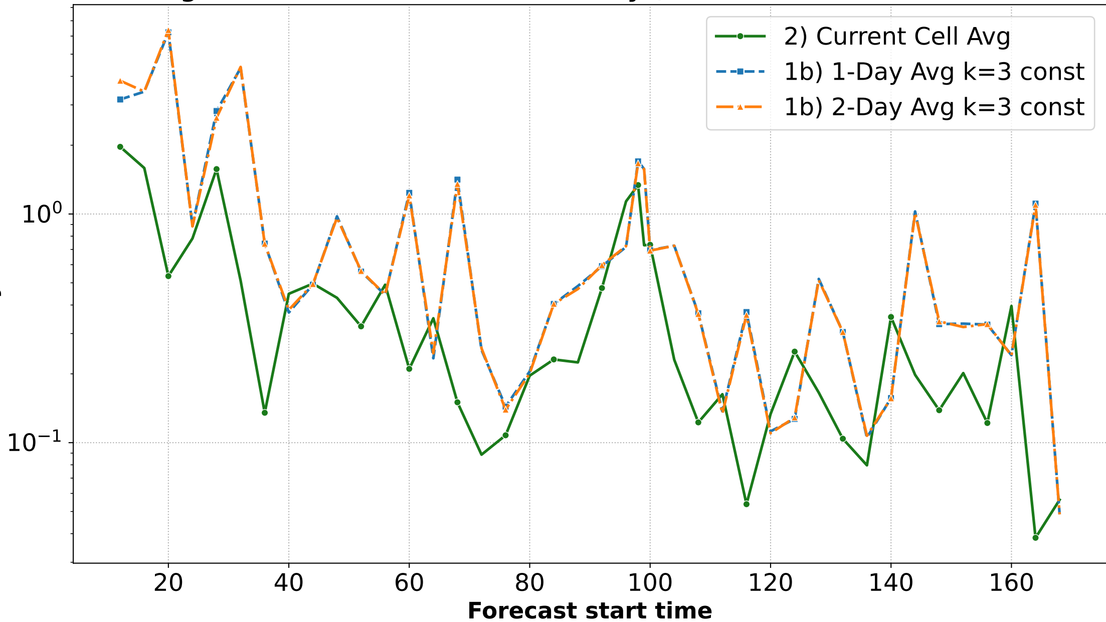
Rolling Forecast Performance (10.0 Days, u_0 shifted to match real data)
