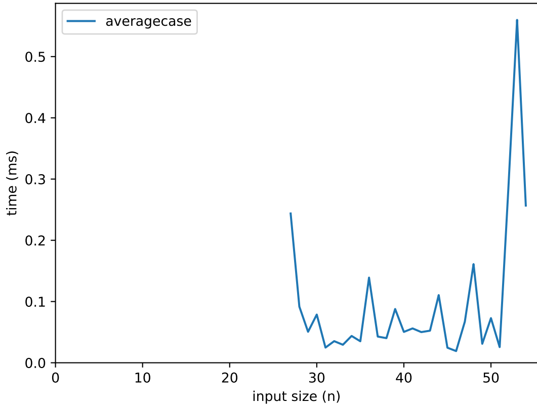
averagecase
