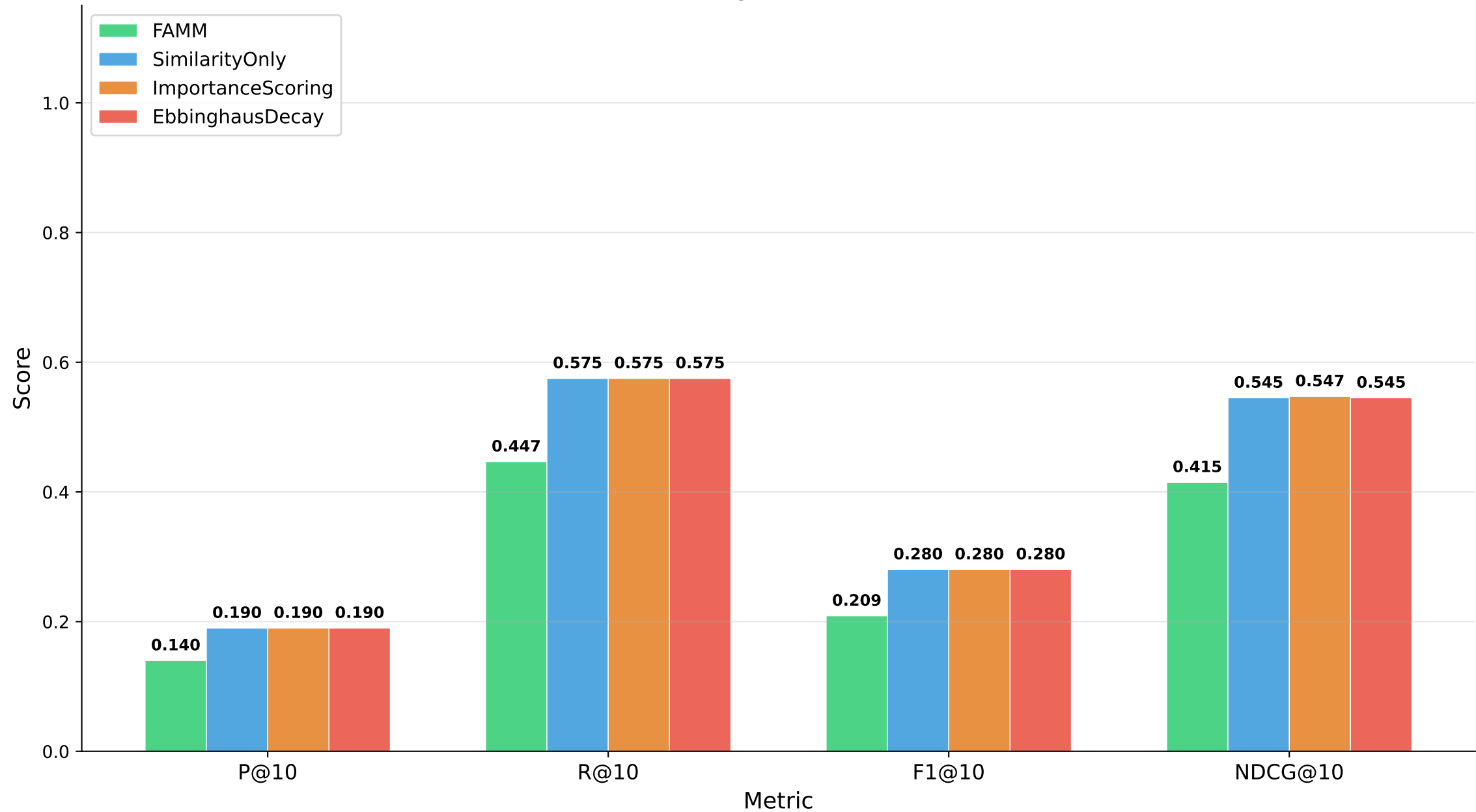
FAMM vs Baselines — Scaled Experiment (100 Memories, 10 Queries)
