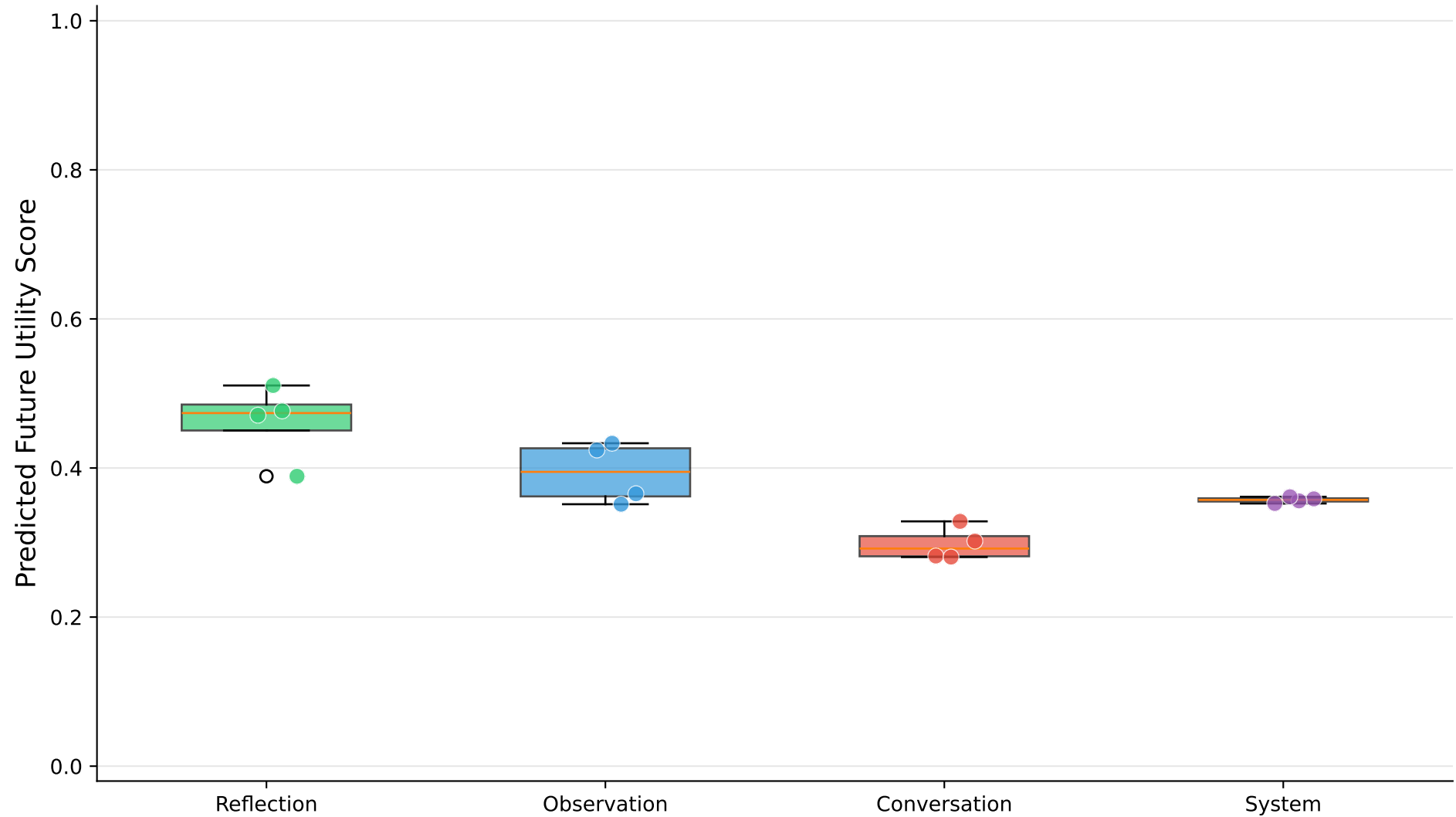
Utility Score Distribution by Memory Source Type
