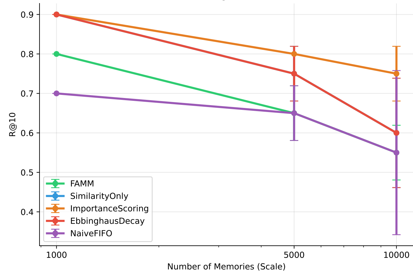
R@10
