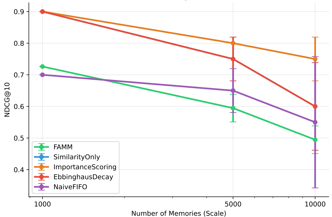
NDCG@10
