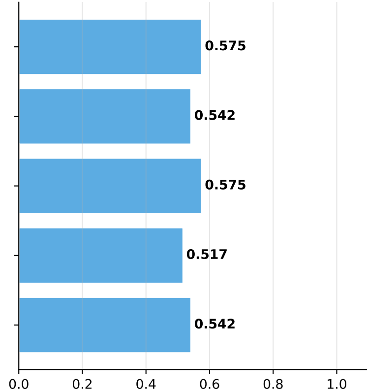
R@10
