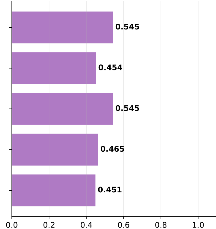
NDCG@10
