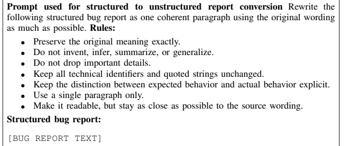
Fig. 4. Prompt template used to convert structured bug reports to unstructured reports.
