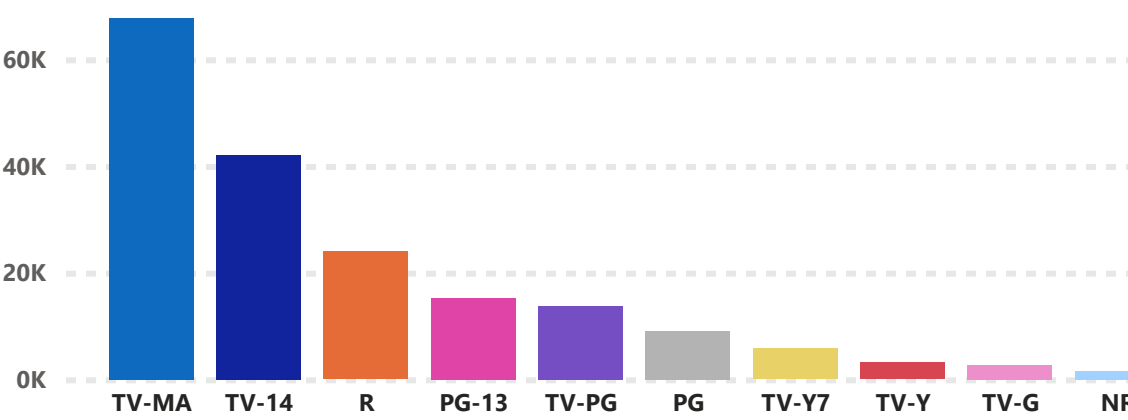
Rating Distribution
