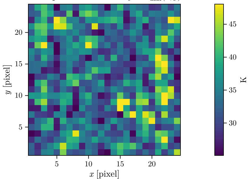
Peak polarized intensity P_{\text{max}}(x, y)
