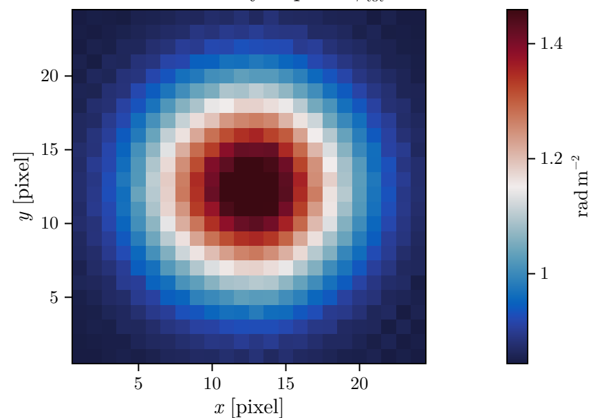
Total Faraday depth \phi_{\text{tot}}
