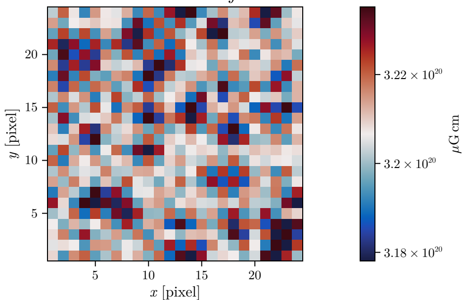
Integrated LOS field \int B_{\text{LOS}} \, dl
