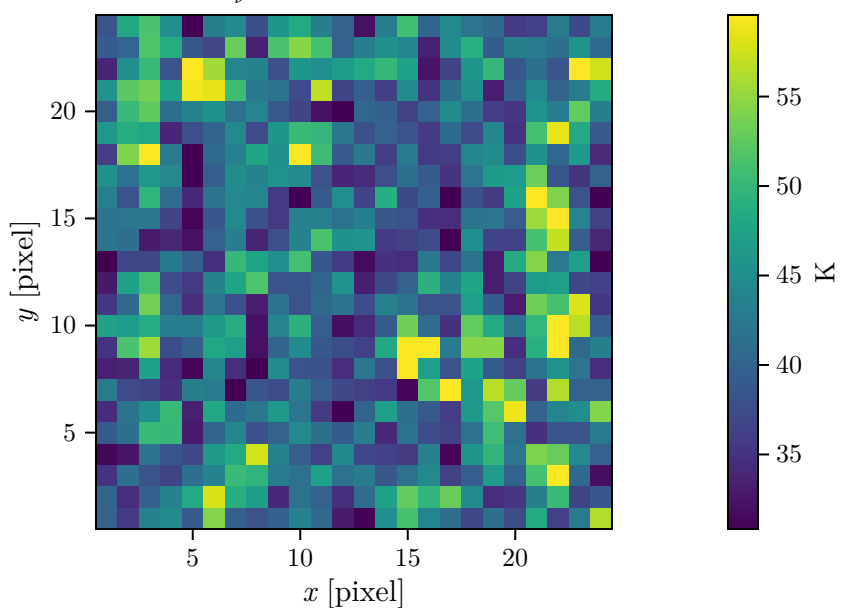
P_\nu \nu = 120.0 \text{ MHz}
