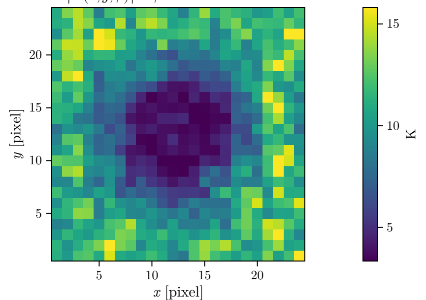
|F(x, y, \phi)| \phi = -20.0 \text{ rad m}^{-2}
