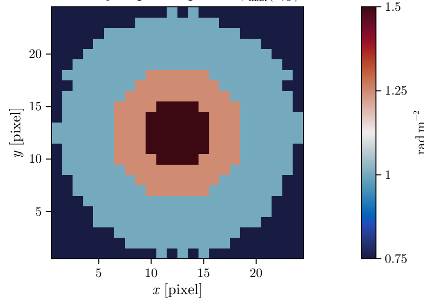
Faraday depth at peak \phi_{\text{max}}(x, y)
