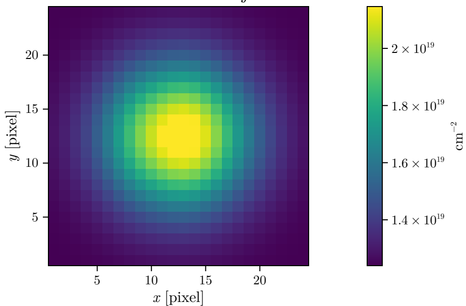
Gas column density \int n \, dl
