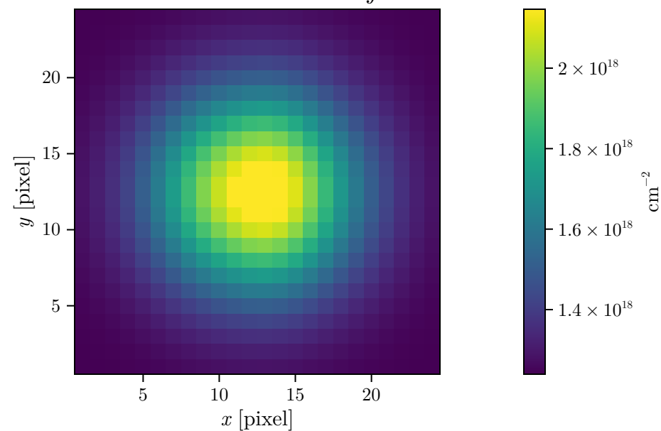
Electron column density \int n_e \, dl
