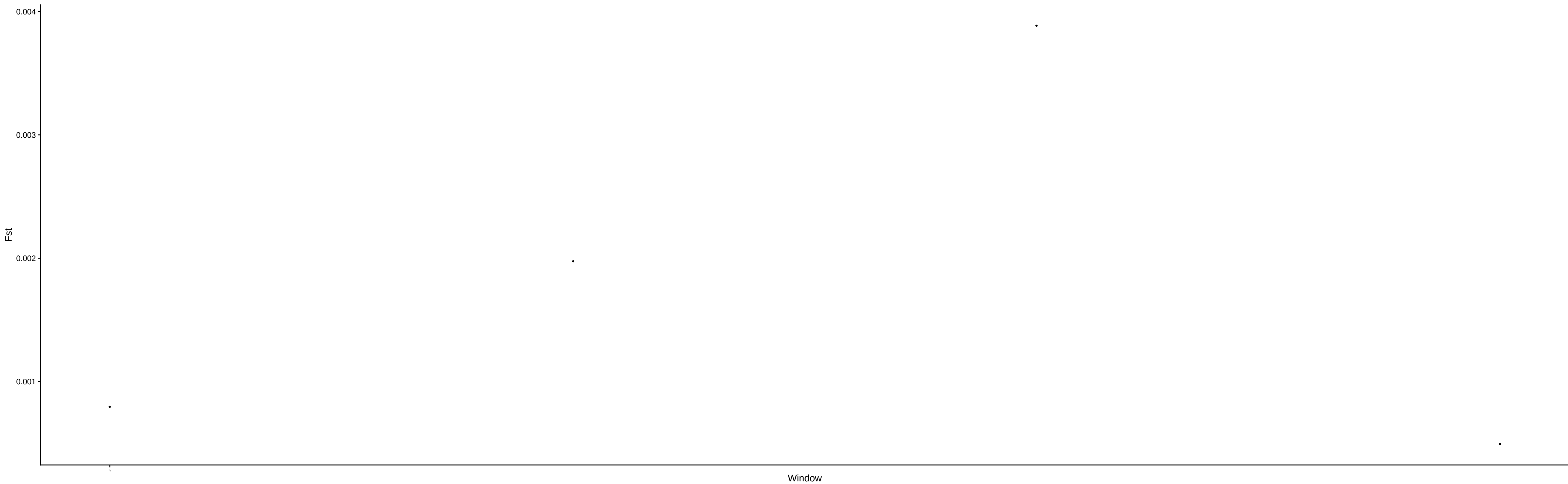
FST for Scaffold: JAKZJL020000194.1
