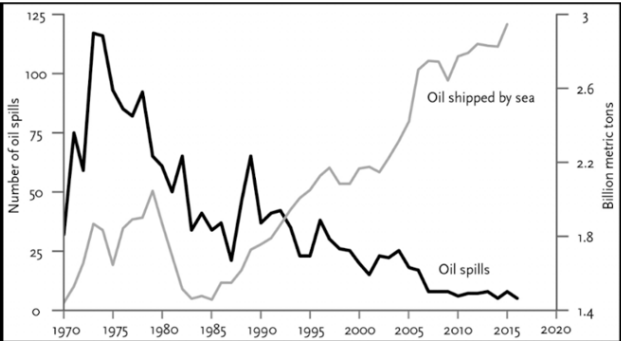
Figure 10-5: Oil spills, 1970–2016
