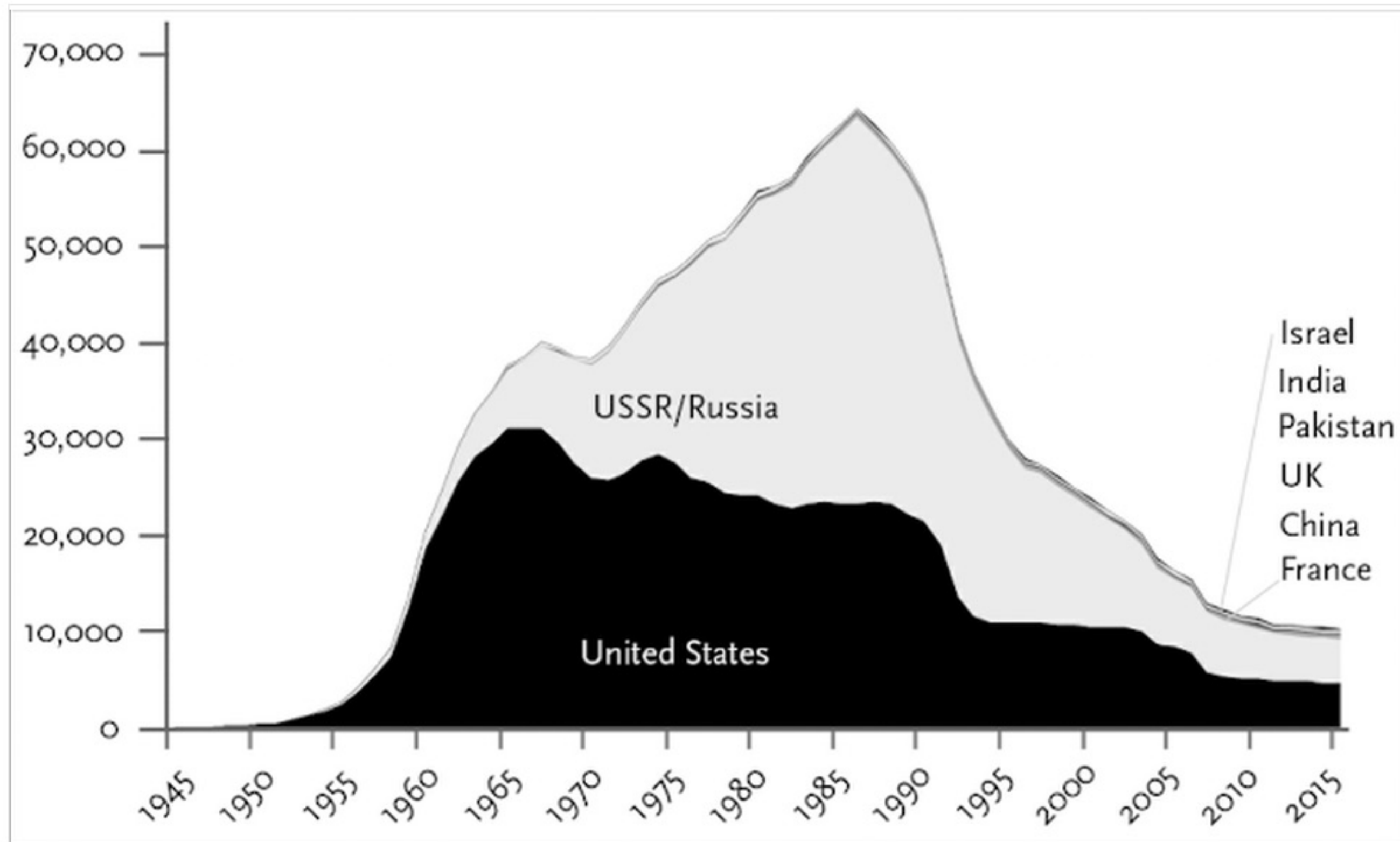
Figure 19-1: Nuclear weapons, 1945-2015
