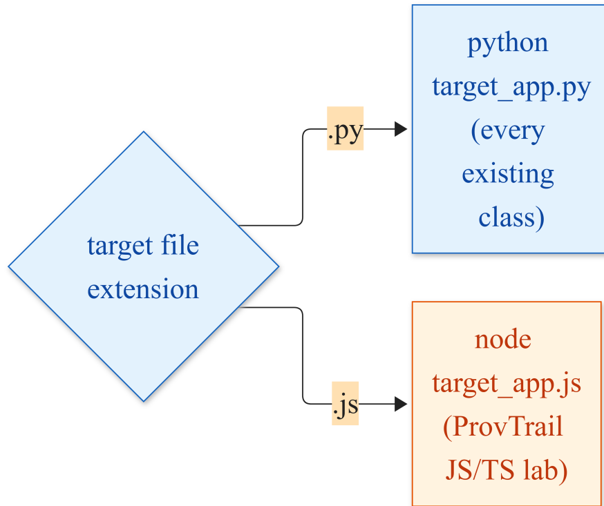
Figure 3.2: The Stage 3.6 interpreter branch: routes execution to python or node depending on target file extension.
