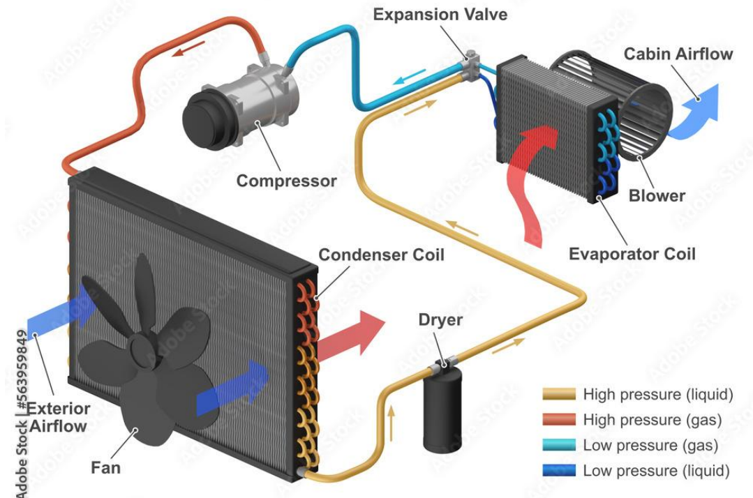
Automotive Air Conditioning System
