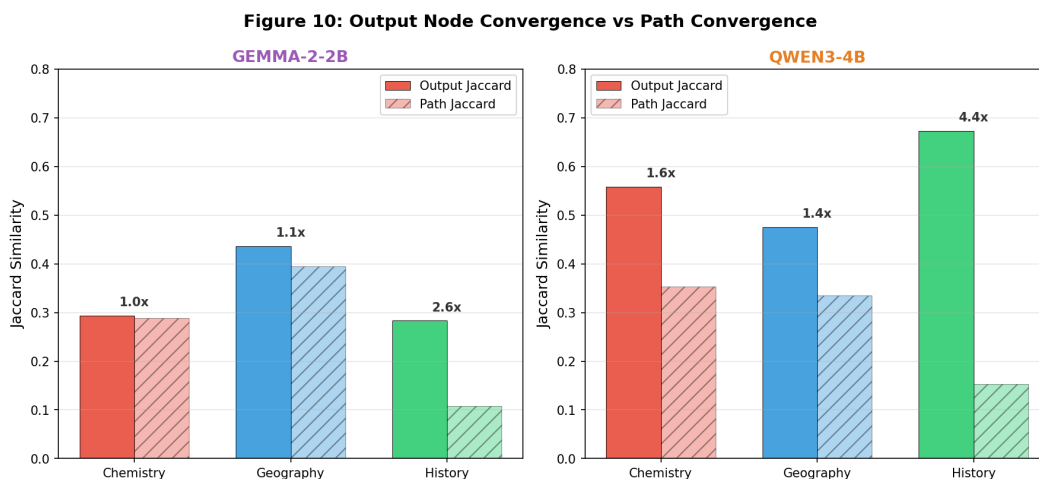
Figure 10: Output node convergence vs path convergence by domain. History shows the largest output/path ratio (4.4x in QWEN).
