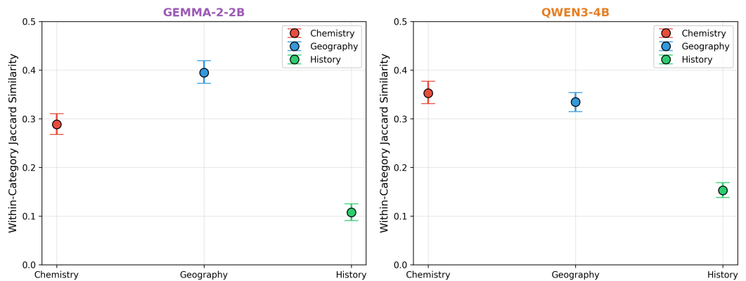
Figure 9: Bootstrap Ci
