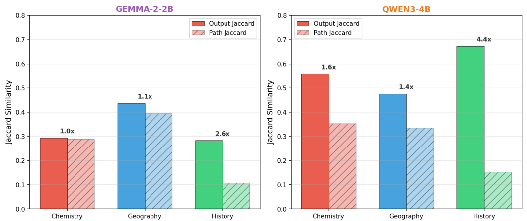
Figure 10: Output Path
