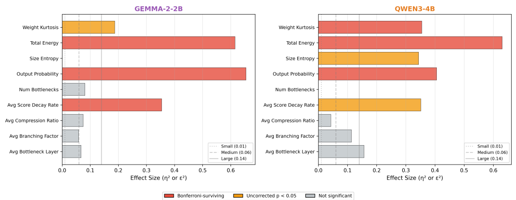
Figure 8: Anova Effects
