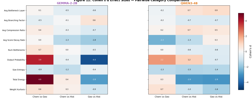
Figure 12: Cohens D
