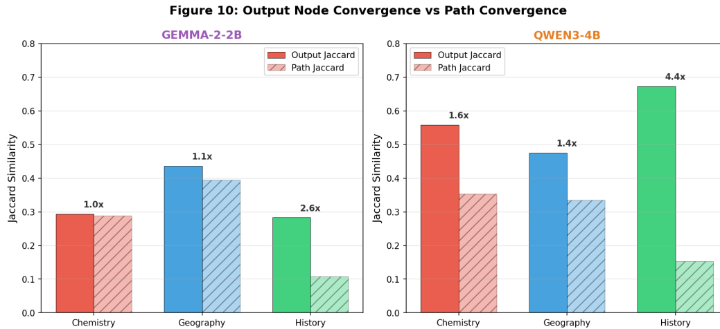
Figure 10: Output node convergence vs path convergence by domain. History shows the largest output/path ratio (4.4× in Qwen).
