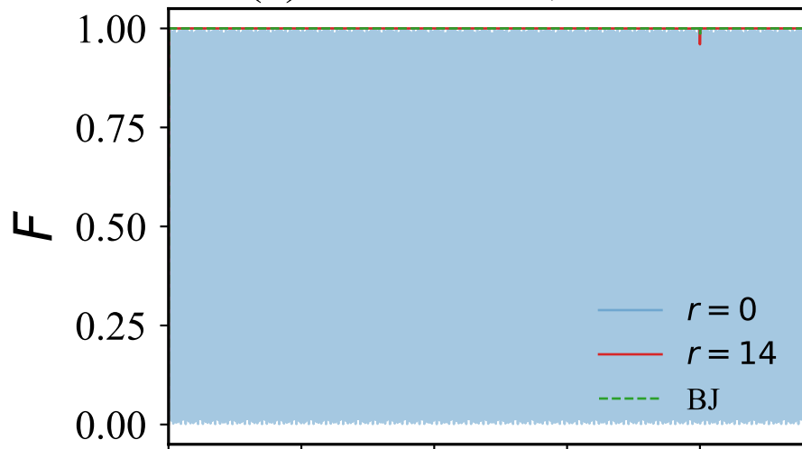
(a) continuous, r = 14
