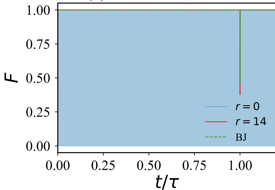
(c) trotterized, r = 14
