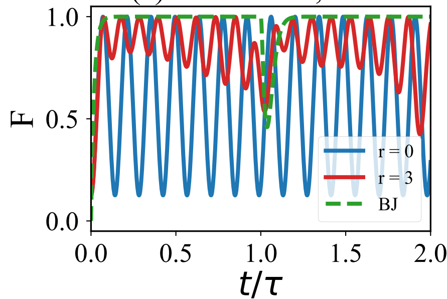
(c) continuous, r = 3
