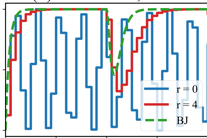
(b) trotterized, r = 4
