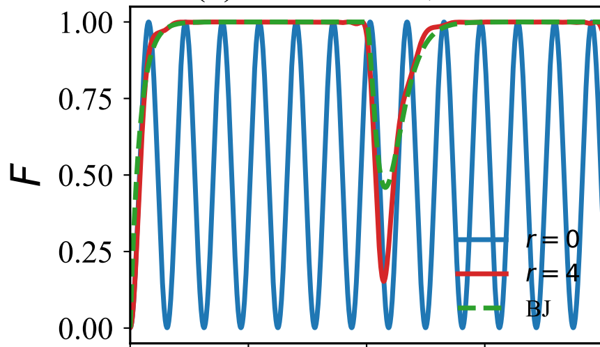
(a) continuous, r = 4
