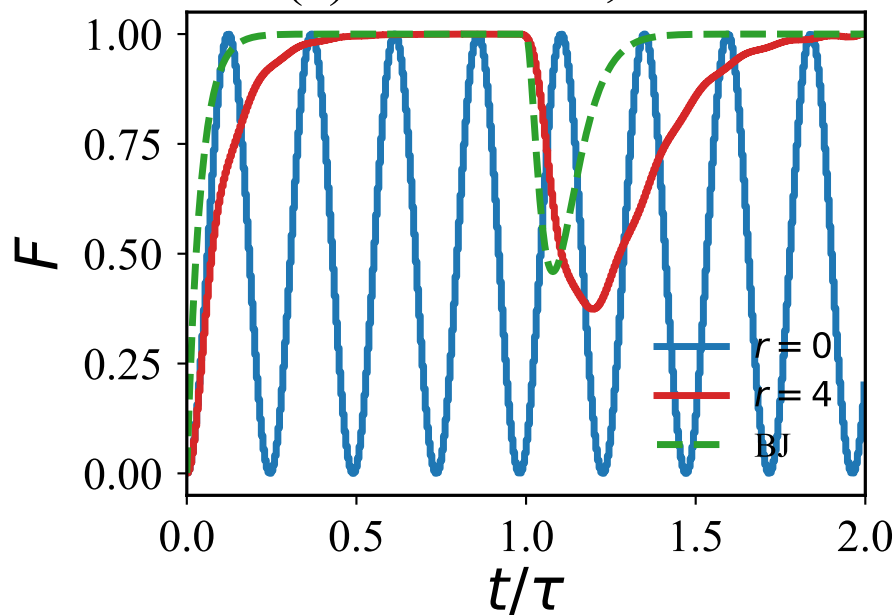
(c) trotterized, r = 4
