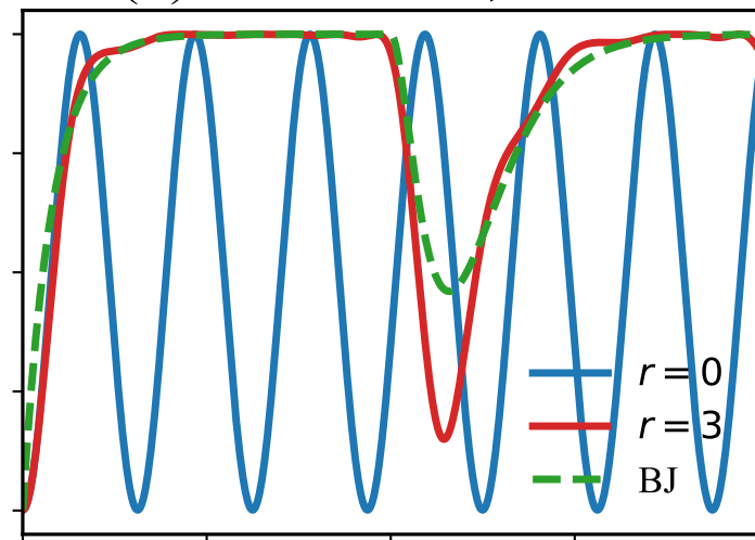
(b) continuous, r = 3
