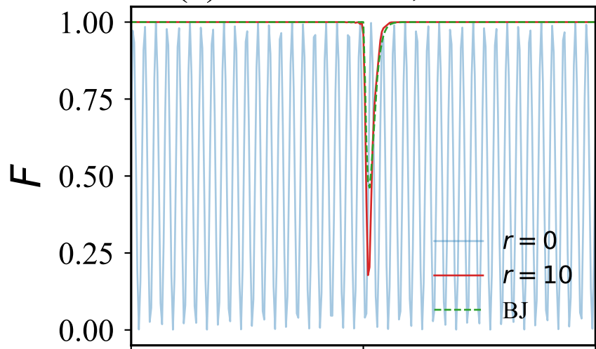
(a) continuous, r = 10
