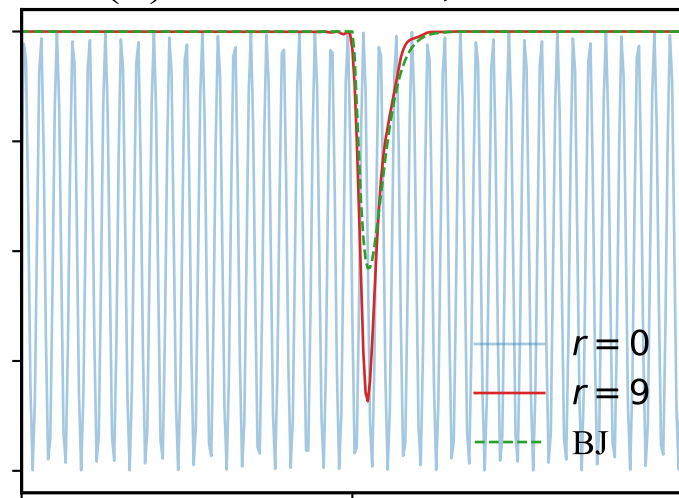
(b) continuous, r = 9
