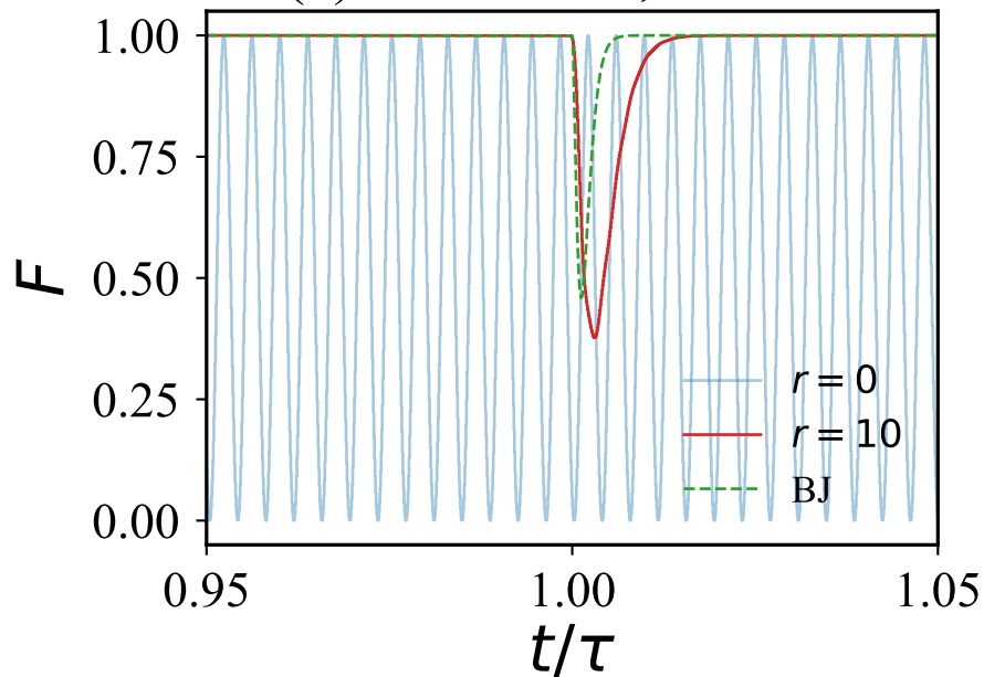
(c) trotterized, r = 10
